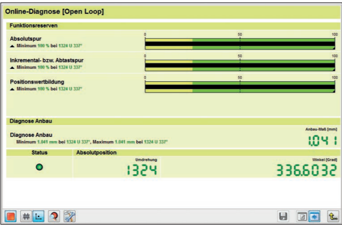
Diagnostics with the PWM 21 and ATS software
