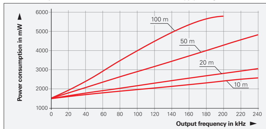
Power consumption (maximum) for the HTLs interface and supply voltage U_P = 30 V
