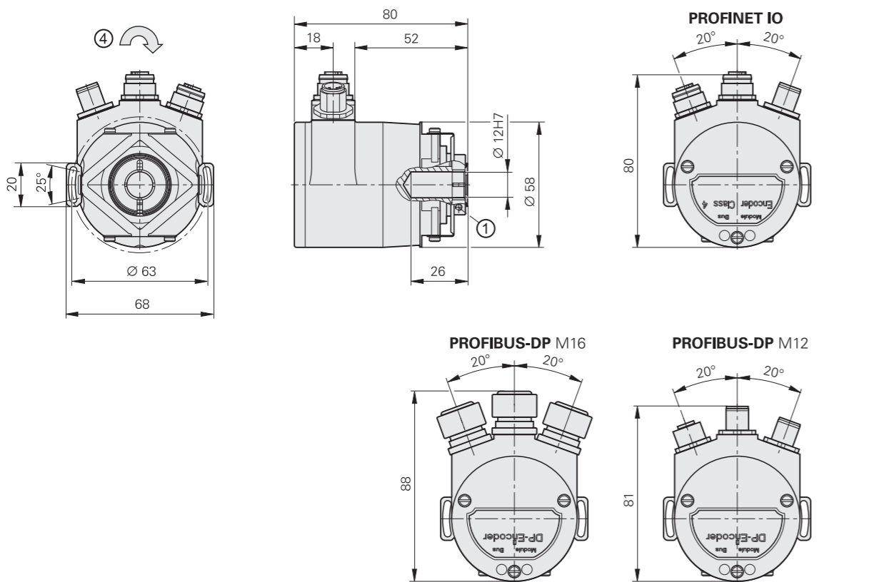
Required mating dimensions
