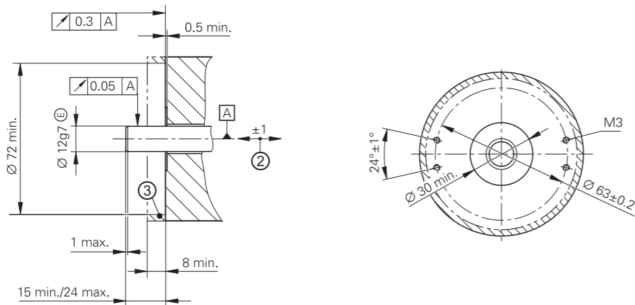
Required mating dimensions
