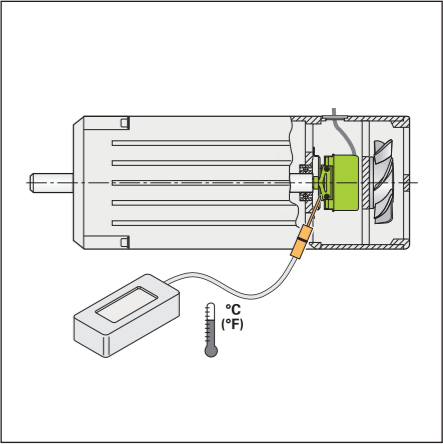
Measuring the actual operating temperature at the defined measuring point of the rotary encoder (see Specifications )
