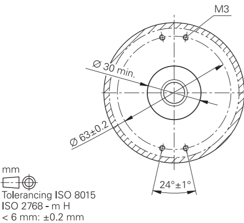
Required mating dimensions
