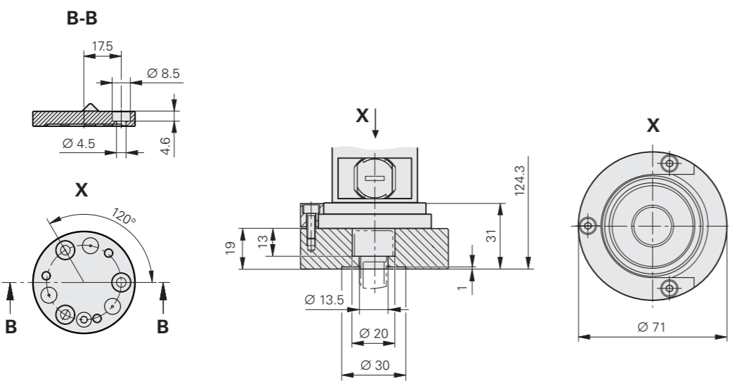
Mounting base
