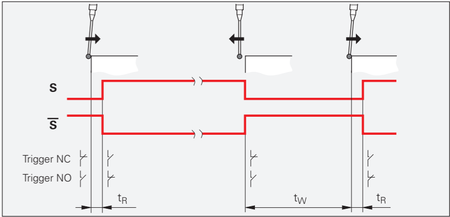
Trigger signal for TS 150/TS 750/TS 260/TT 160
